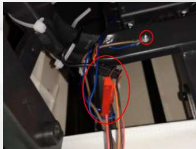
8.断开端子并拆卸1颗地线螺丝 Disconnect the terminal and remove one ground screw.
